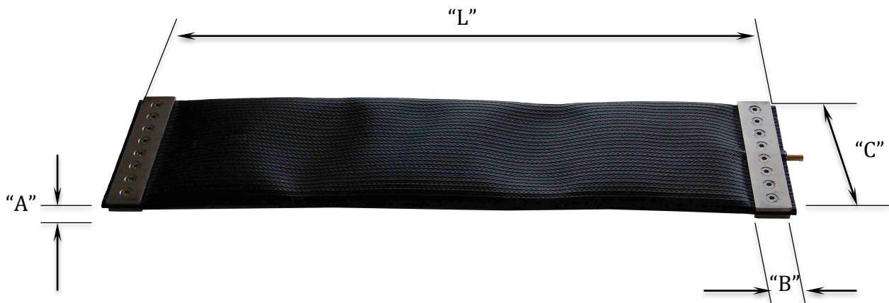
Type ESV Vertical threaded conn. V-D-1/4" (D1) or V-D-1/2" (D2)
