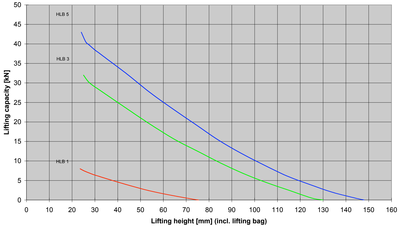
Lifting capacity / Lifting height-diagram HLB-range (at 8 bar)
