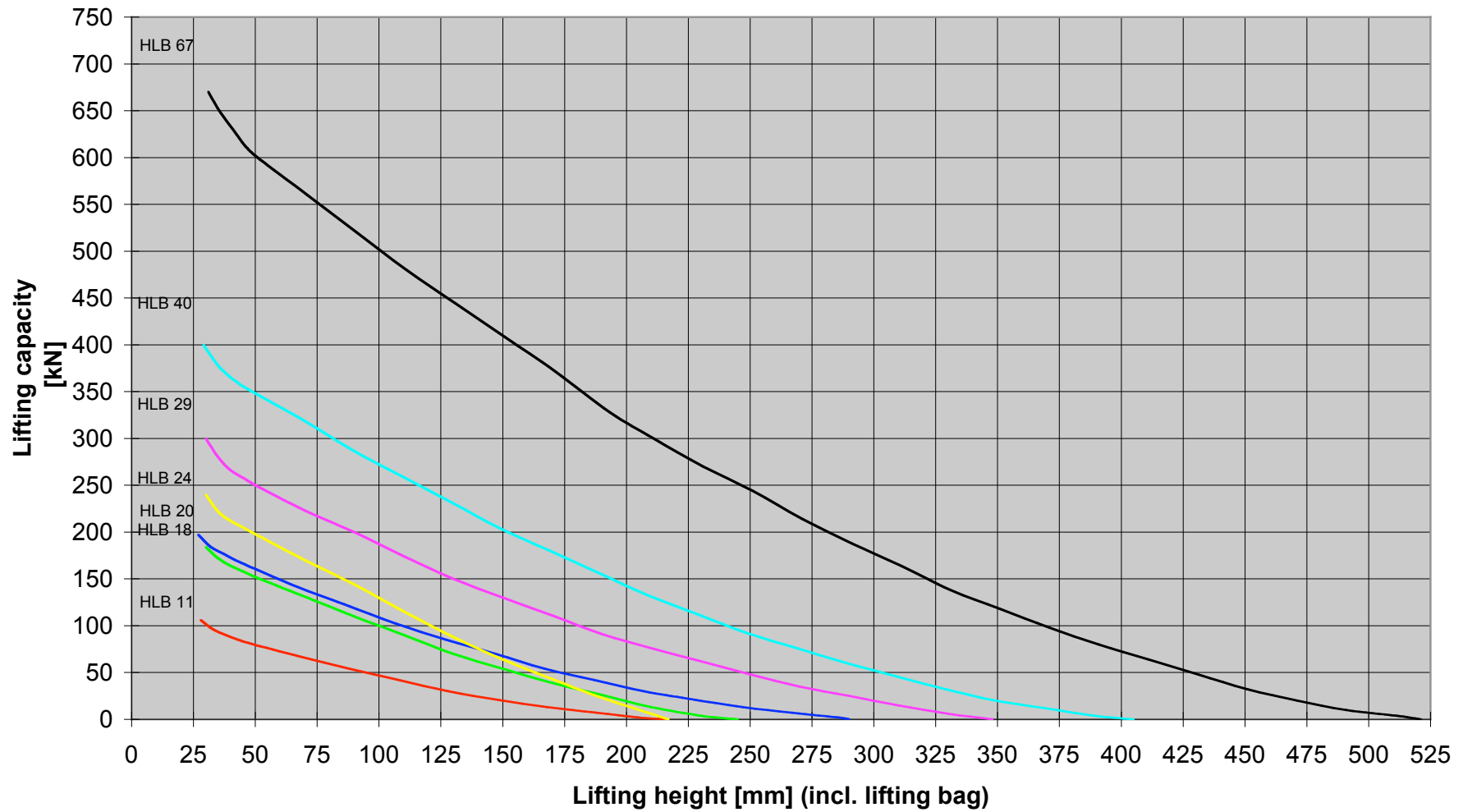
Lifting capacity / Lifting height-diagram HLB-range (at 8 bar)
